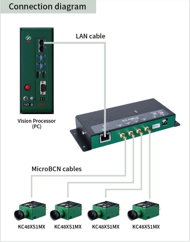
4ch CXP to GigE Multiplexer
